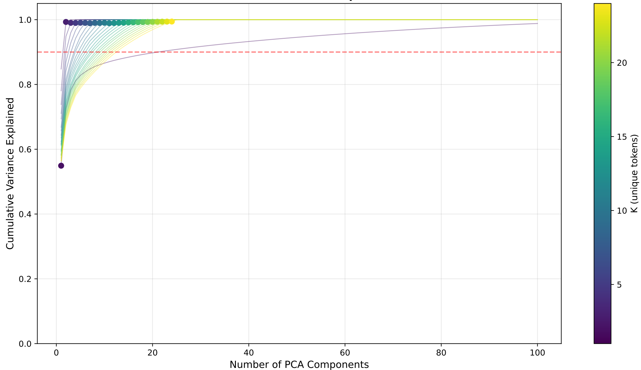
PCA Cumulative Variance Curves by K (mlp_hidden, step 20000) Dots mark the K-th component
