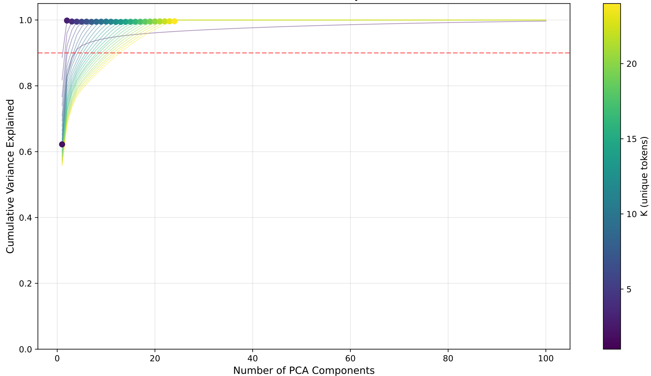
PCA Cumulative Variance Curves by K (post_In2, step 20000) Dots mark the K-th component
