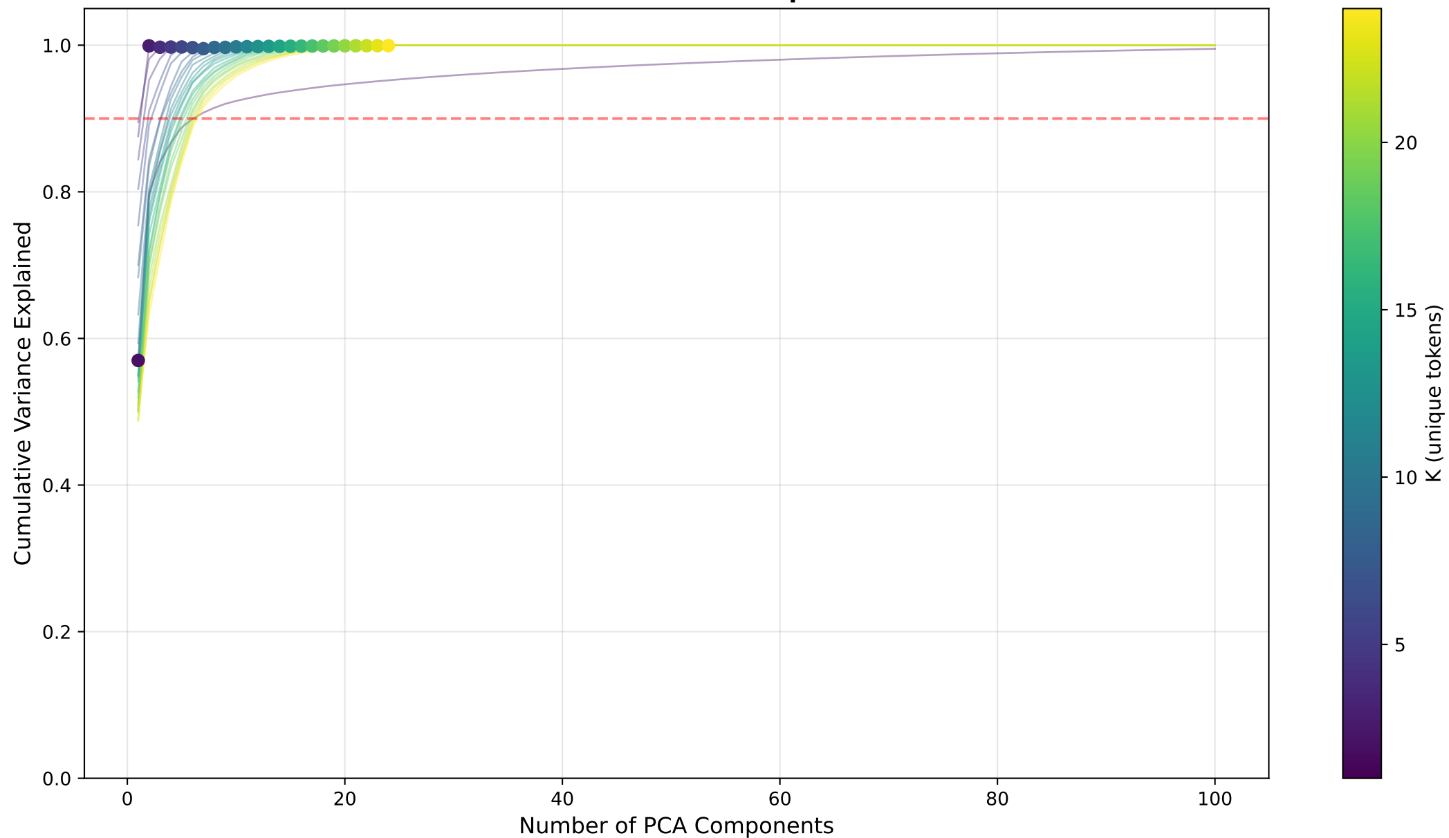
PCA Cumulative Variance Curves by K (post_mlp, step 20000) Dots mark the K-th component
