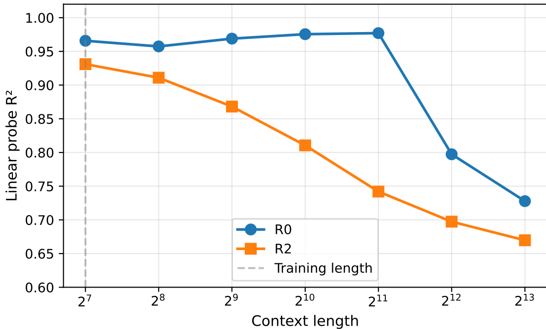
Position Decoding Extrapolation
