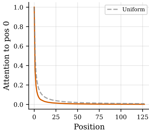
(b) Attention to Position 0
