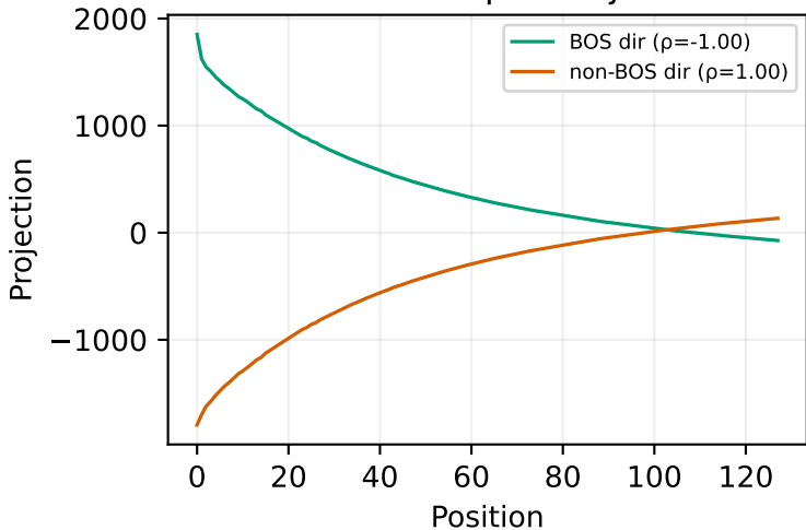
Attention Output Projection
