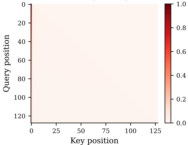
Block 2 (Trained)
