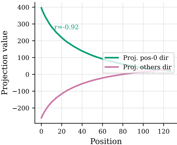
Attention Output Projection
