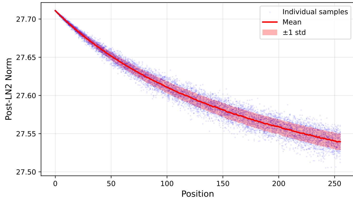
Post-LN2 Norm vs Position ( r = -0.9679 )
