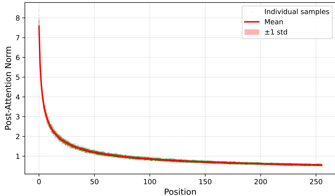
Post-Attention Norm vs Position ( r = -0.6587 )
