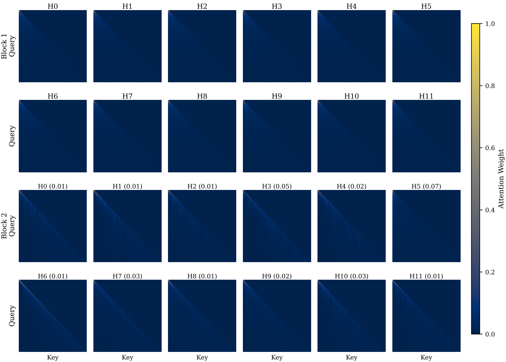
R1: Full Attention Maps (Block 1 top, Block 2 bottom) * indicates BOS head (>50% attention to position 0)
