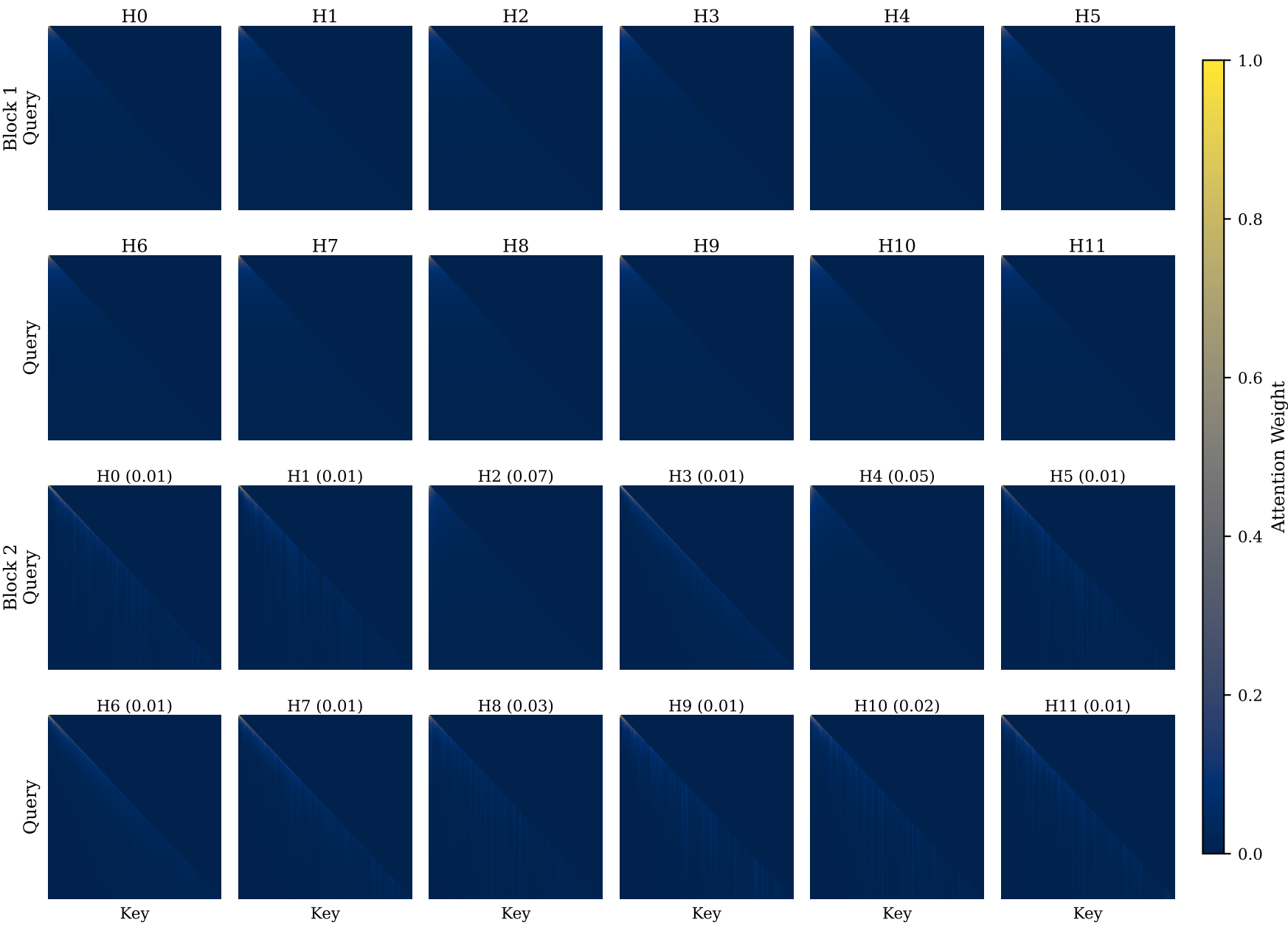
R2: Full Attention Maps (Block 1 top, Block 2 bottom) * indicates BOS head (>50% attention to position 0)
