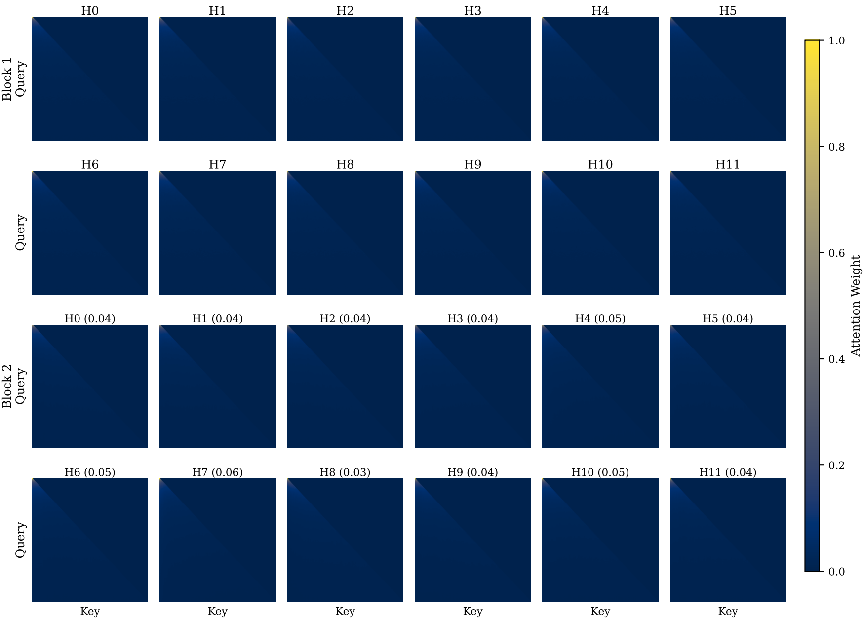
R3: Full Attention Maps (Block 1 top, Block 2 bottom) * indicates BOS head (>50% attention to position 0)
