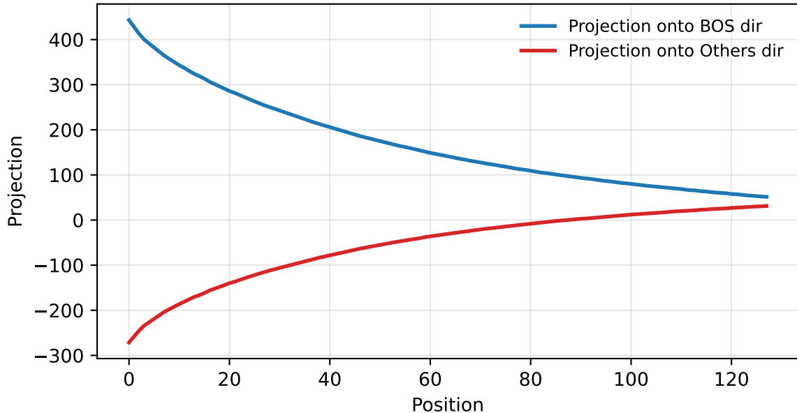
Attention Output Projection
