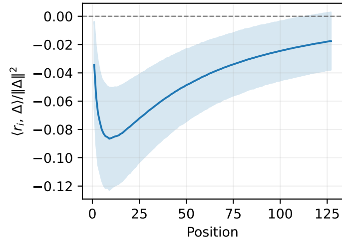
Projected Residual
