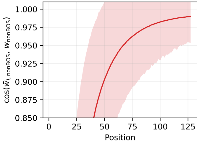
Non-BOS Concentration
