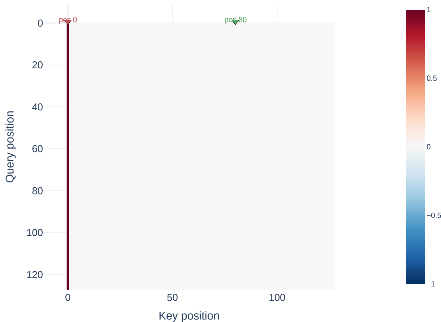
Head 7 attention after softmax (mean over samples)
