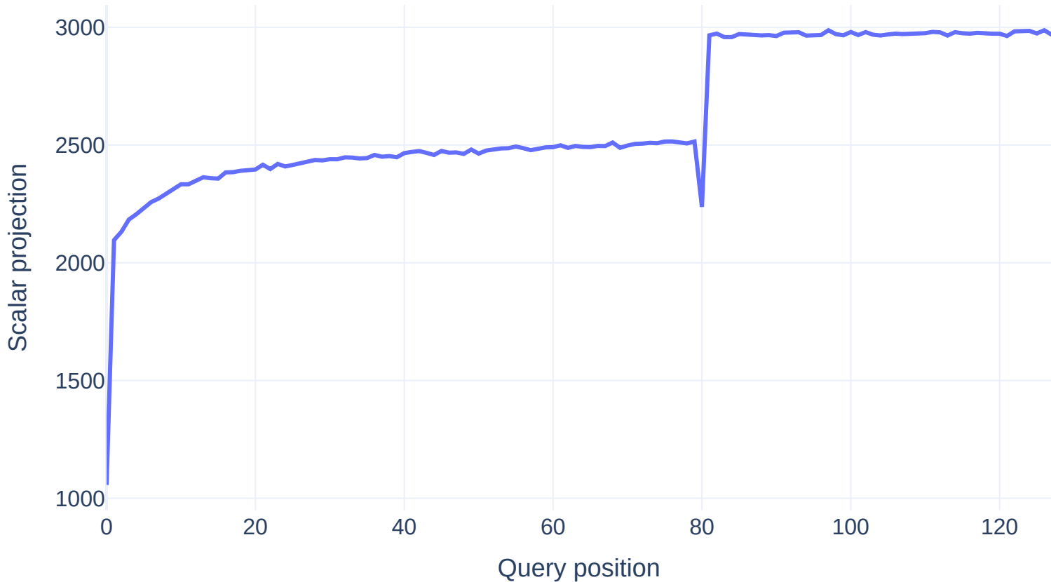
Head 7 scalar projection: q_t \cdot k_0 (mean over samples)
