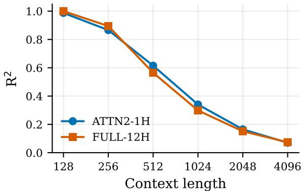
(b) Head fine-tune (frozen backbone)
