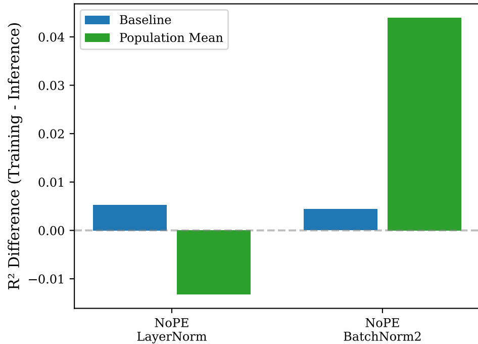
Mode Difference (Train vs Eval)
