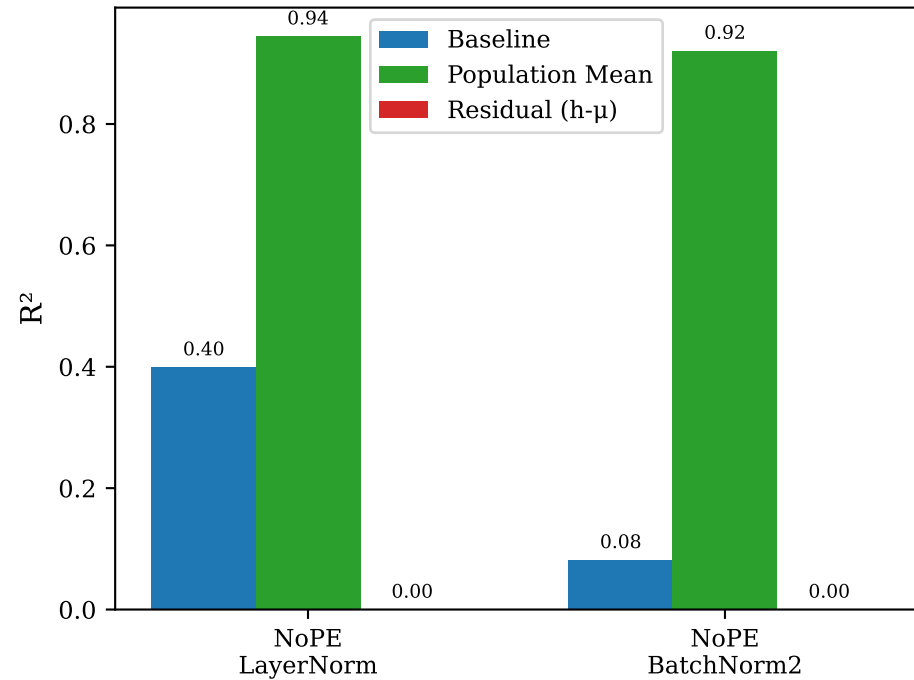
Population Statistics Probing
