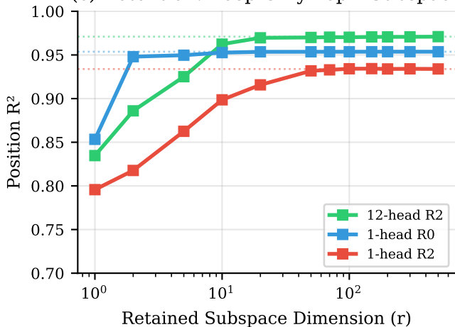
(c) Retention: Keep Only Top-r Subspace
