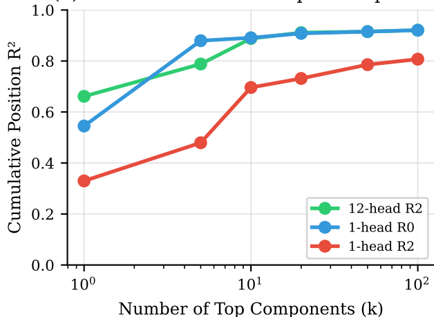
(b) Cumulative R^2 from Top-k Components
