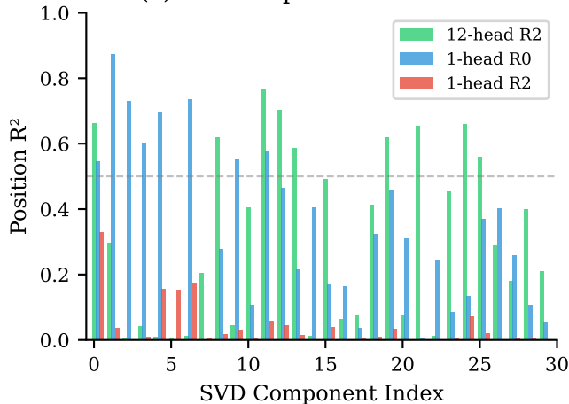
(a) Per-Component Position R^2
