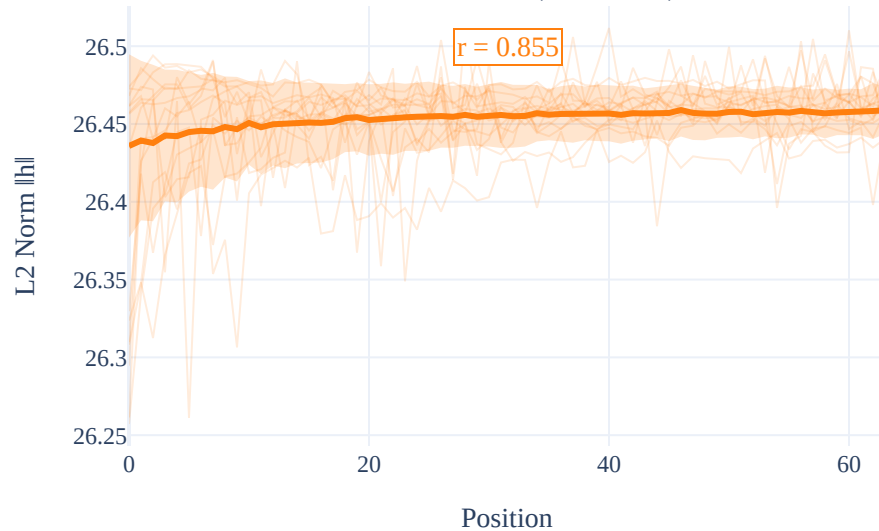
Trained Model (Post-LN2)
