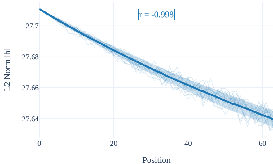
Random Model (Post-LN2)
