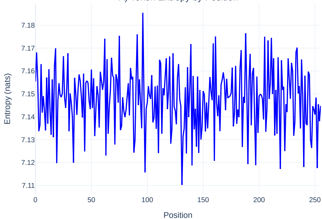
A) Token Entropy by Position
