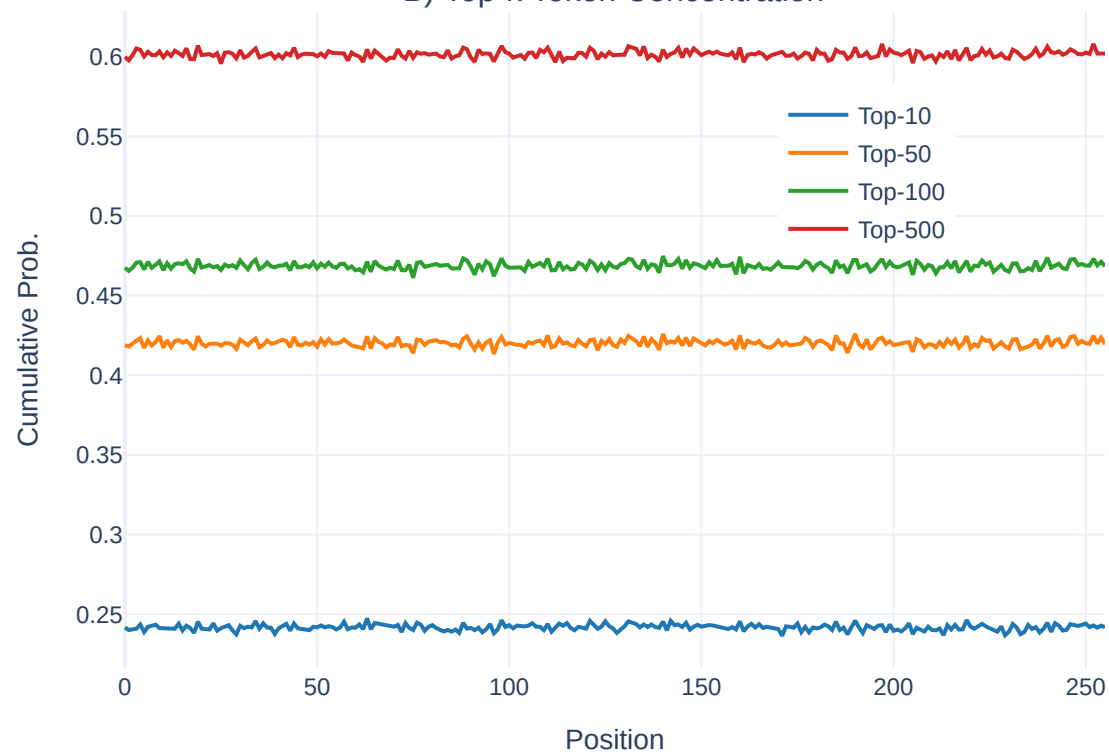
B) Top-k Token Concentration
