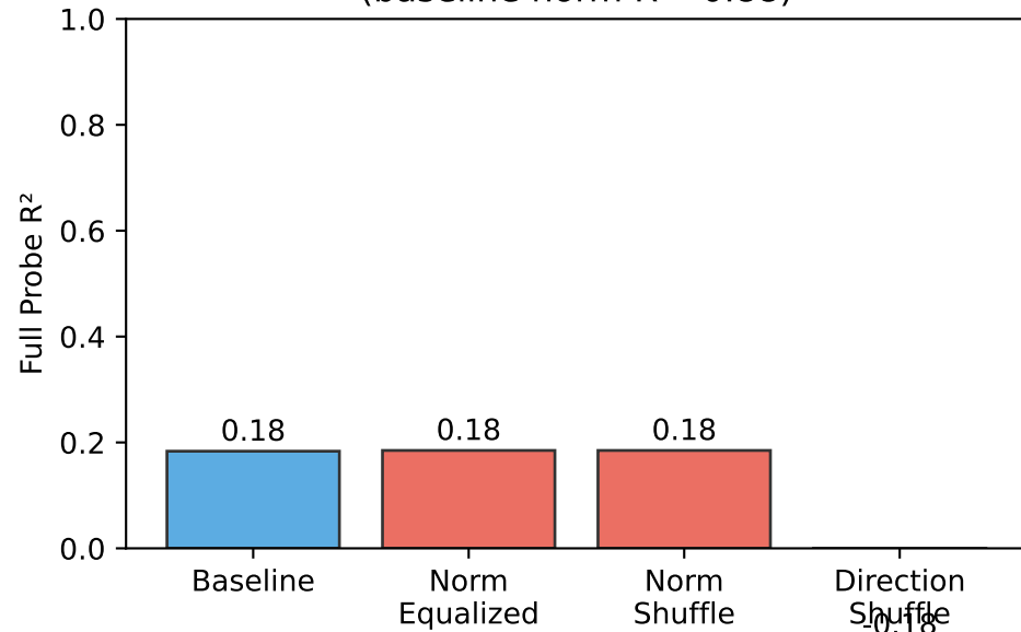
synthetic_small (baseline norm R^2=0.88 )
