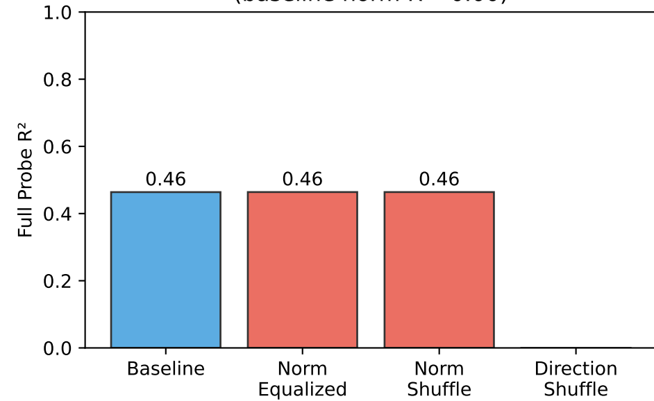
trained_shakespeare (baseline norm R^2=0.00 )
