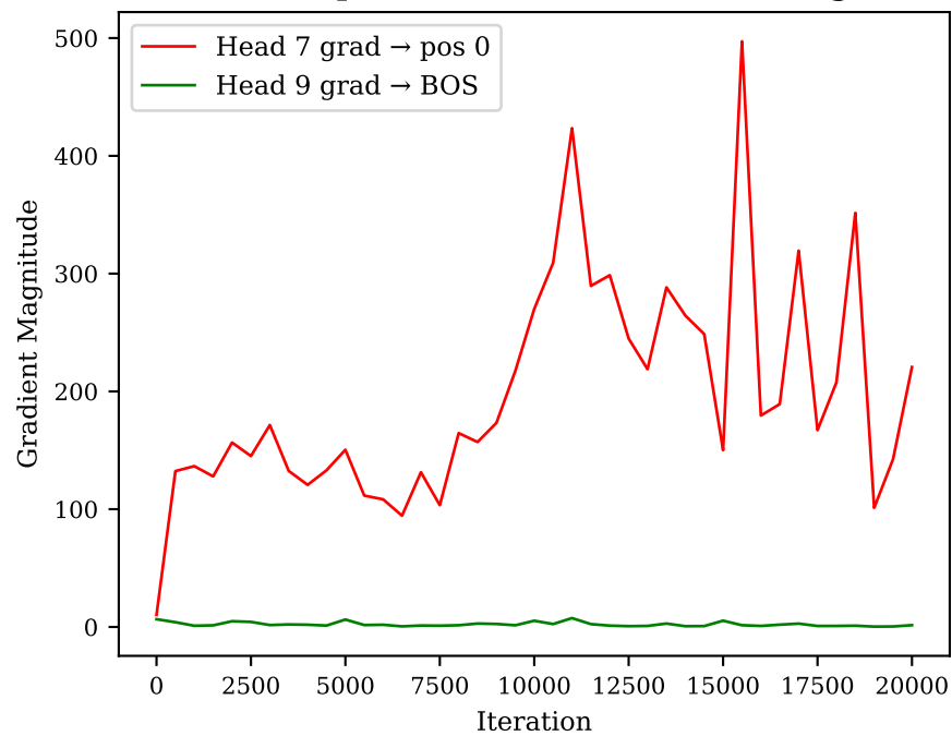
Head-Specific Gradients Over Training
