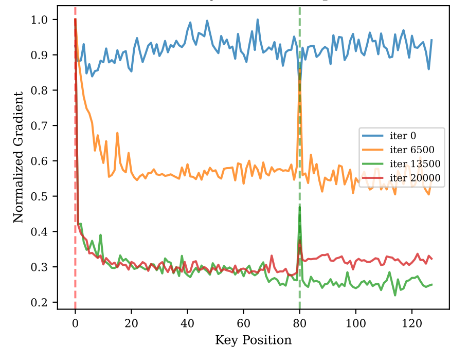
Gradient by Position (snapshots)
