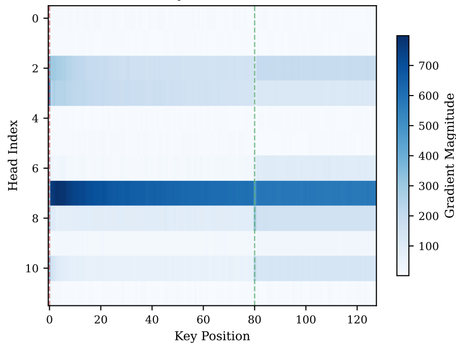
Gradient by Head and Position
