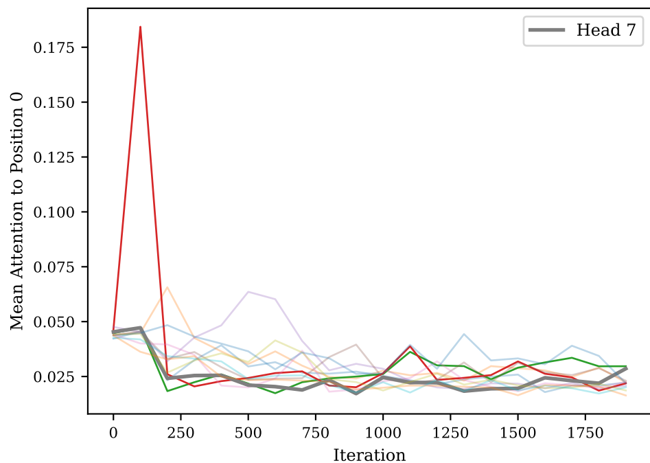
Block 2: All Heads → Position 0
