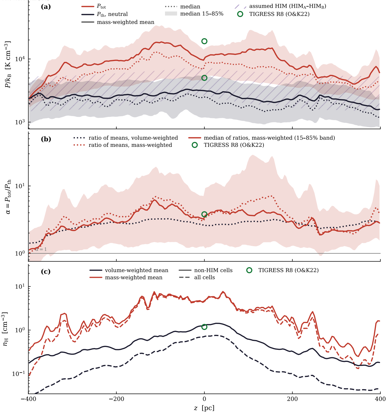
TIGRESS R8 has \Sigma_{\text{gas}} \approx 9.9 \text{ M}_{\odot} \text{ pc}^{-2} , about twice the local value — absolute pressures are not expected to match; \alpha can.
