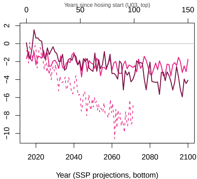
IPSL-CM6A-LR
