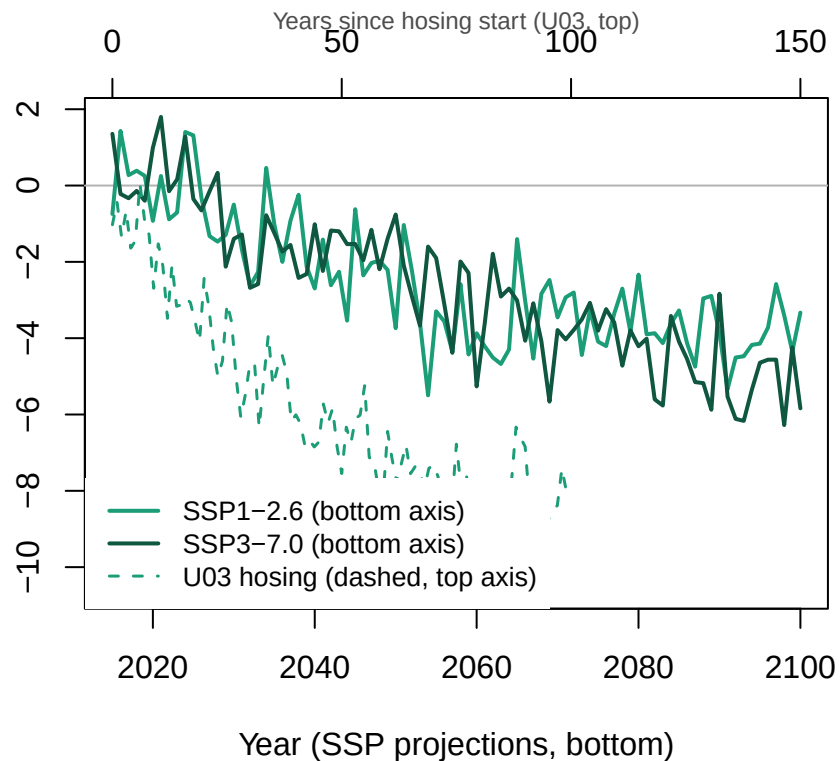
EC-Earth3
