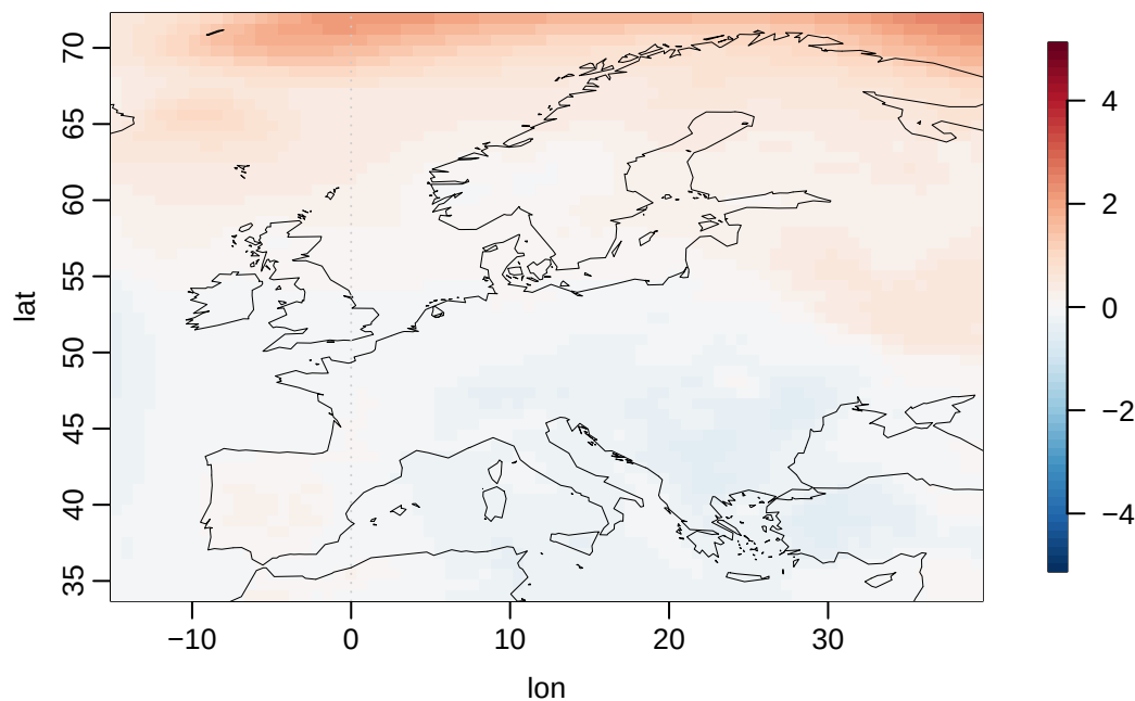
HadGEM3-GC31-LL g01 (Europe mean -0.74)
