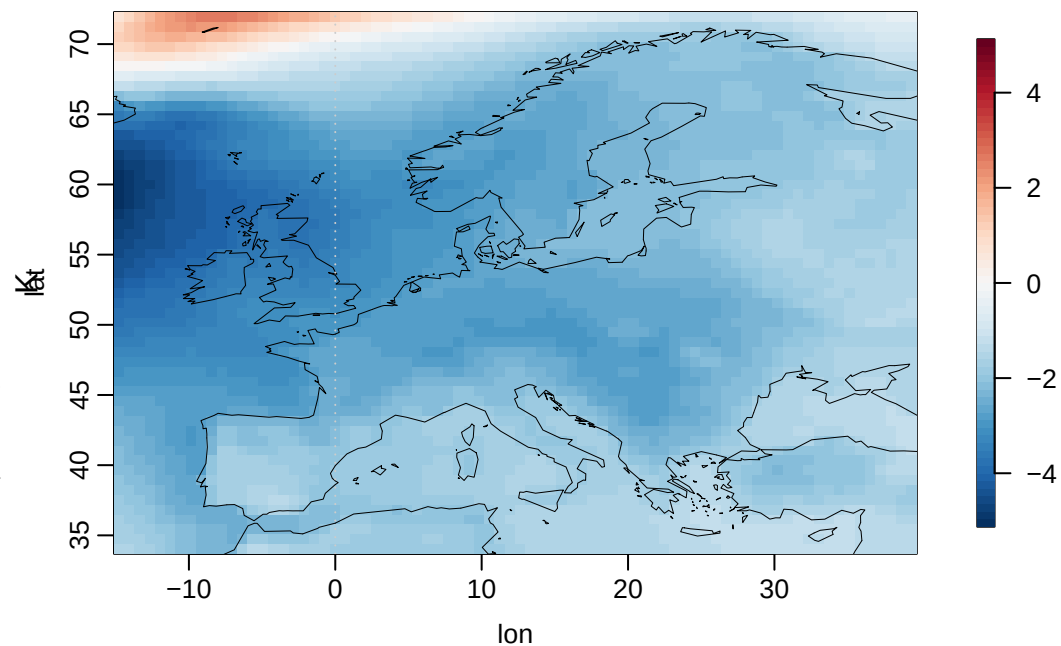
HadGEM3-GC31-MM g01 (Europe mean -1.96)
