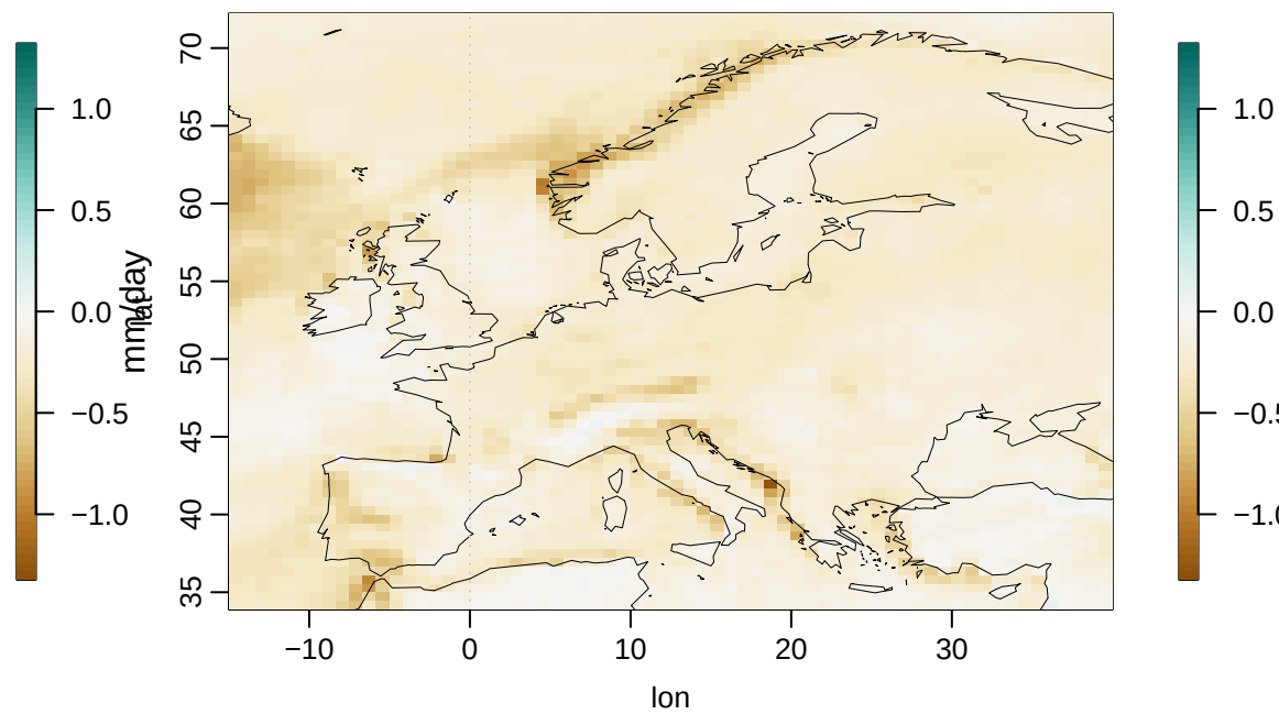
HadGEM3-GC31-MM g01 (Europe mean -0.23)
