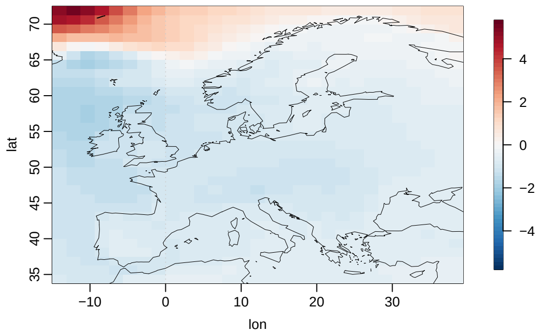
HadGEM3-GC31-LL g01 (Europe mean -0.71)
