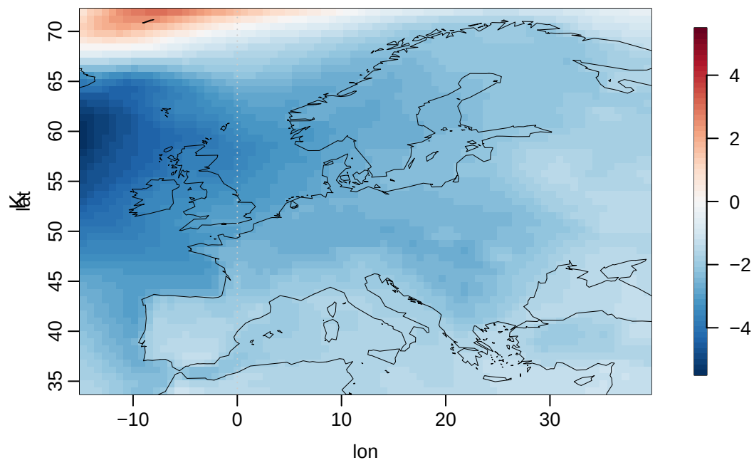
HadGEM3-GC31-MM g01 (Europe mean -2.06)
