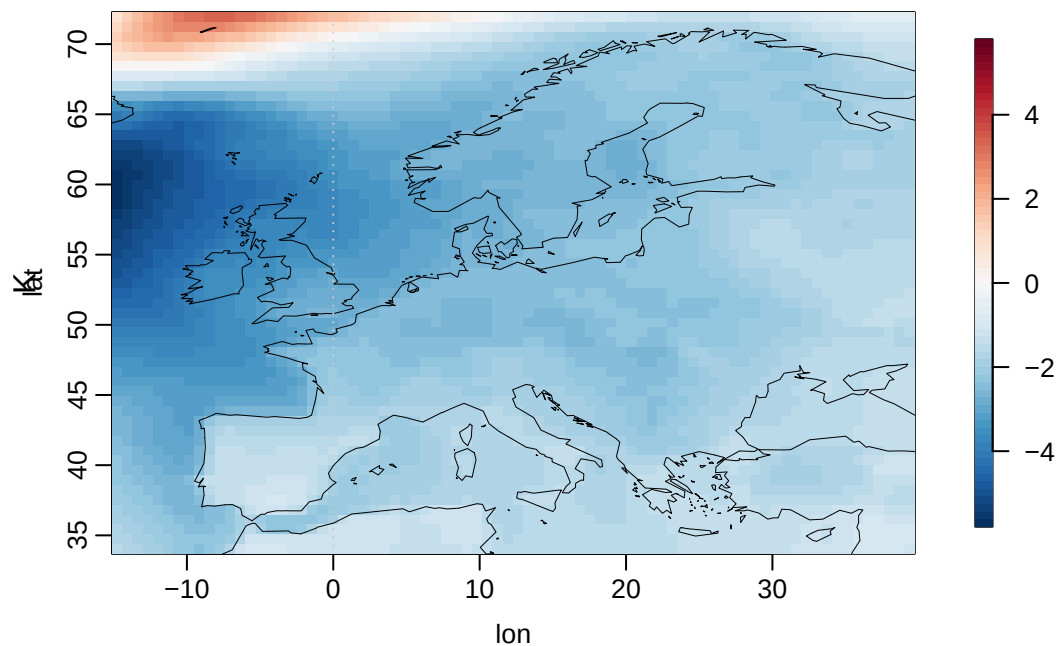
HadGEM3-GC31-MM g01 (Europe mean -2.21)
