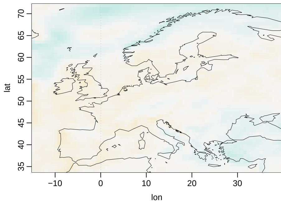
HadGEM3-GC31-LL g01 (Europe mean -0.11)
