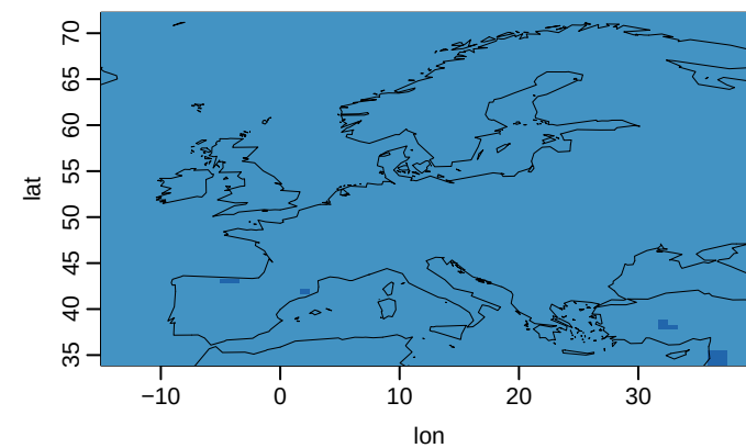
HadGEM3-GC31-MM u03 (yr 67-100) CW 0% CD 100% HD 0% HW 0%
