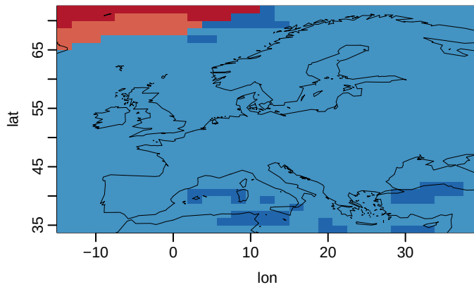
IPSL-CM6A-LR u03 (yr 51–100) CW 3% CD 97% HD 0% HW 0%
