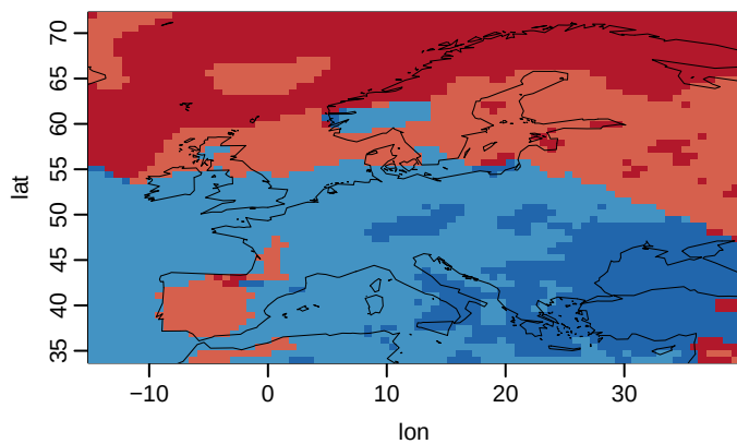
HadGEM3-GC31-LL u03 (yr 67-100) CW 3% CD 95% HD 1% HW 0%
