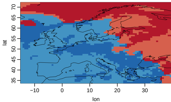
HadGEM3-GC31-LL u03 (yr 1-33) CW 9% CD 87% HD 0% HW 4%
