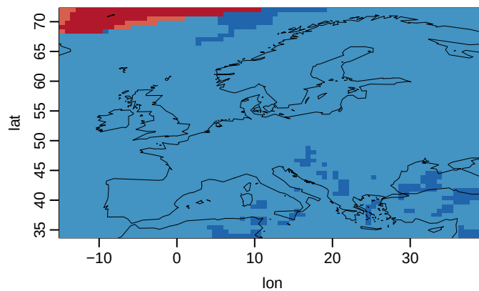
HadGEM3-GC31-MM g01 (yr 67-100) CW 1% CD 99% HD 0% HW 0%
