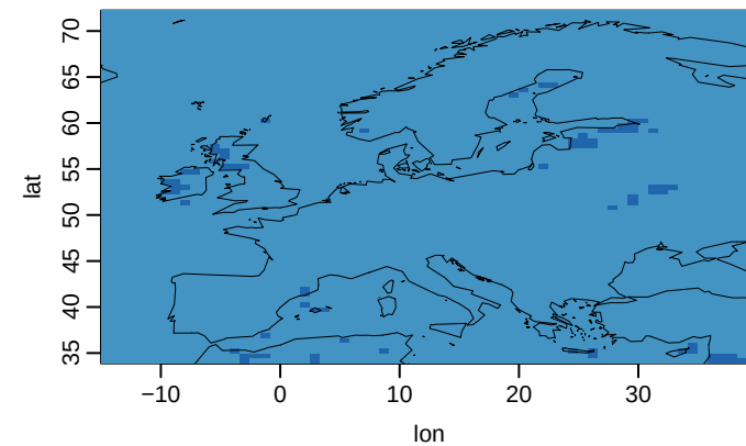
HadGEM3-GC31-MM u03 (yr 1-33) CW 2% CD 98% HD 0% HW 0%
