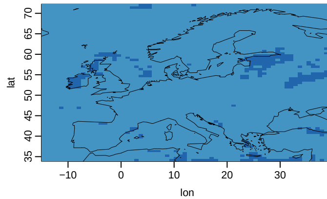
HadGEM3-GC31-MM g01 (yr 34–66) CW 6% CD 94% HD 0% HW 0%
