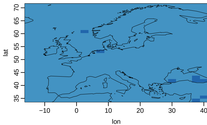
IPSL-CM6A-LR u03 (yr 101-150) CW 1% CD 99% HD 0% HW 0%
