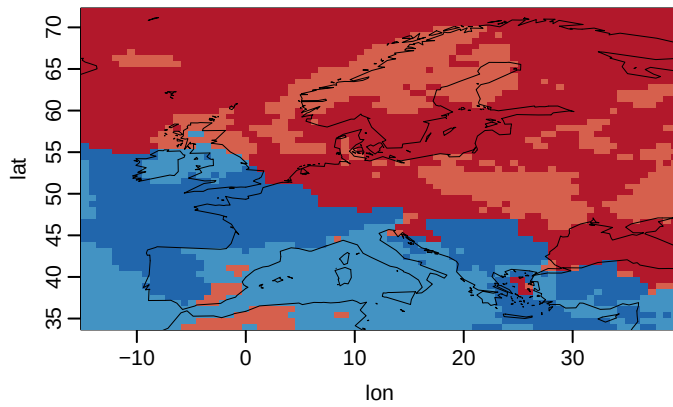
HadGEM3-GC31-LL u03 (yr 34–66) CW 6% CD 91% HD 2% HW 1%
