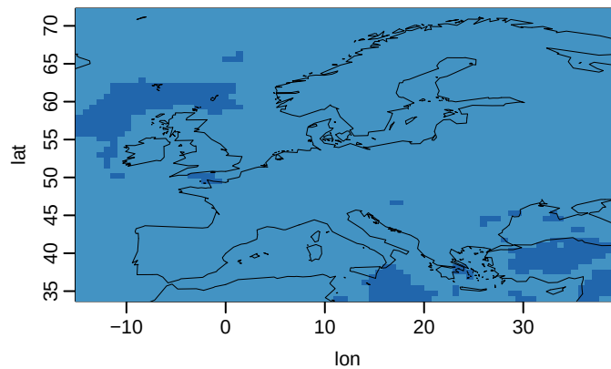
HadGEM3-GC31-MM g01 (yr 1-33) CW 35% CD 53% HD 10% HW 3%
