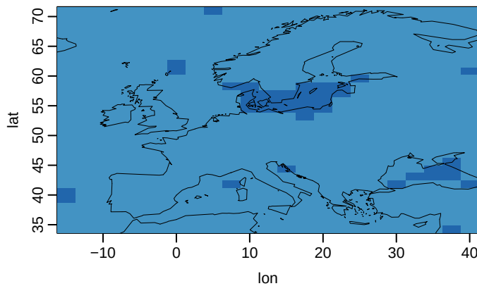
IPSL-CM6A-LR u03 (yr 1-50) CW 6% CD 94% HD 0% HW 0%
