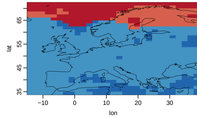
HadGEM3-GC31-MM u03 (yr 34–66) CW 0% CD 100% HD 0% HW 0%
