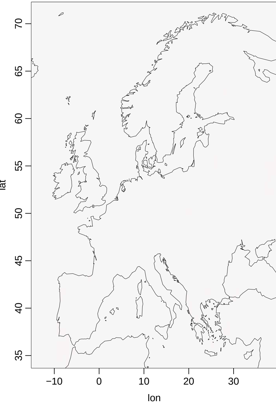
g01: % hosing months outside piControl range
