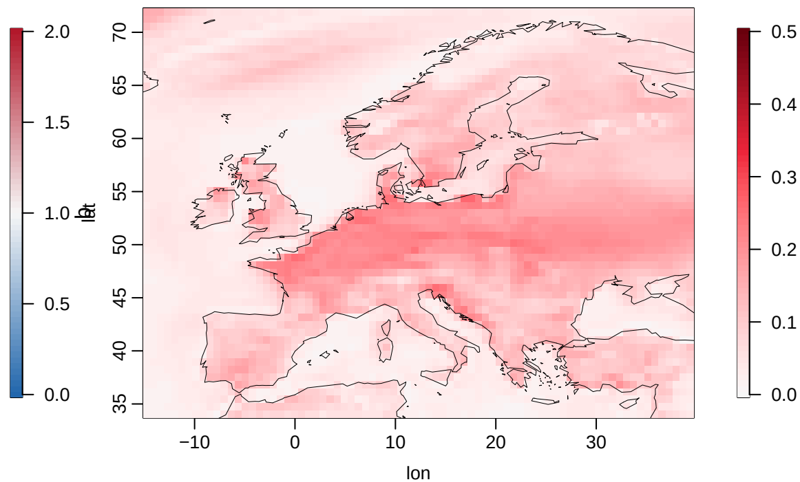
tasmax slope spread across months (MAD)
