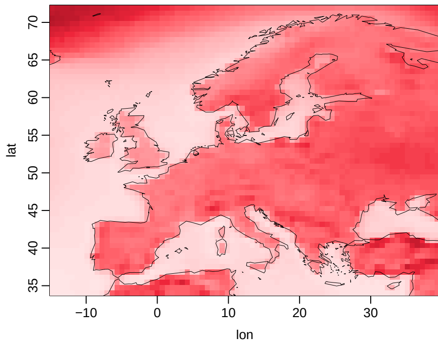
tasmax RMSE, median month [K]
