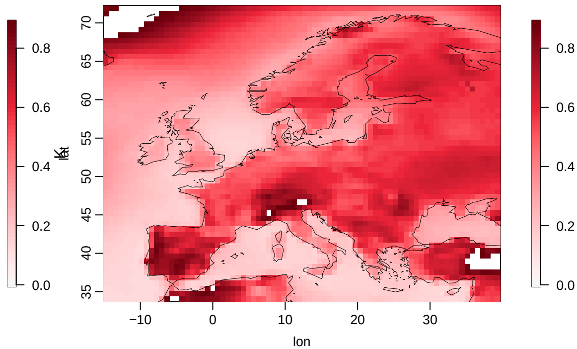
tasmax RMSE, worst month [K]
