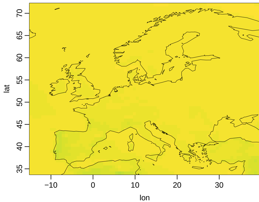
tasmax R2, median month
