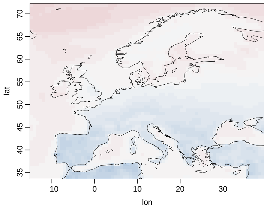
tasmax slope b, median month
