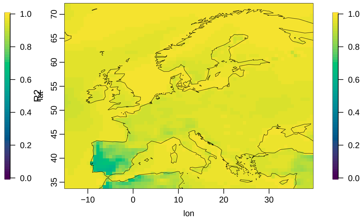
tasmax R2, worst month
