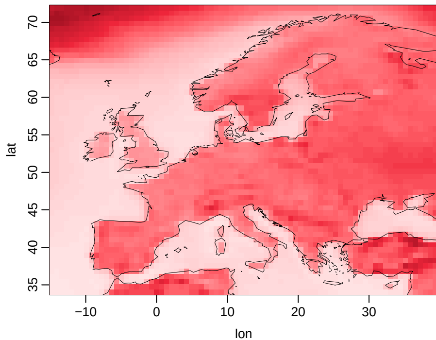
tasmax OUT-of-sample RMSE [K]
