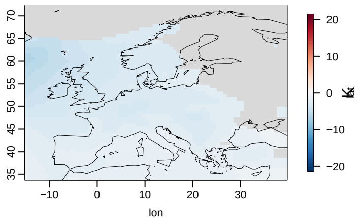
HadGEM3-GC31-MM g01
