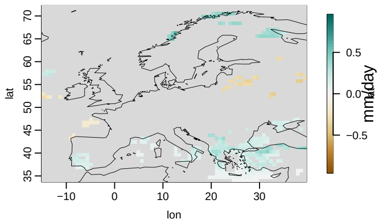
HadGEM3-GC31-LL u03
