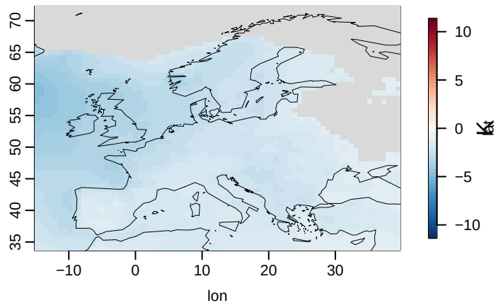
HadGEM3-GC31-MM g01
