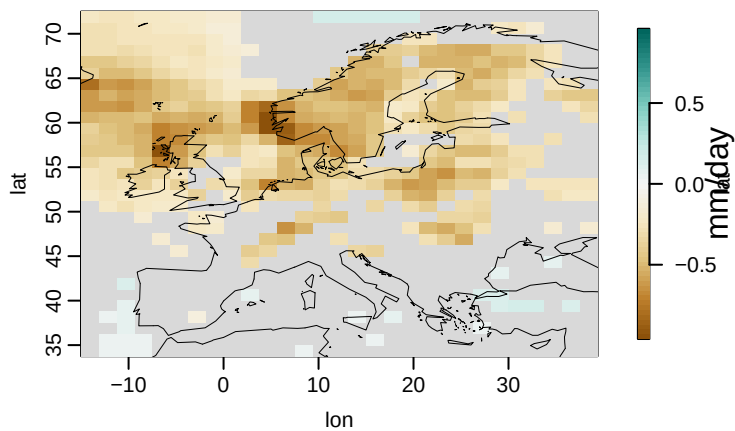
IPSL-CM6A-LR u03
