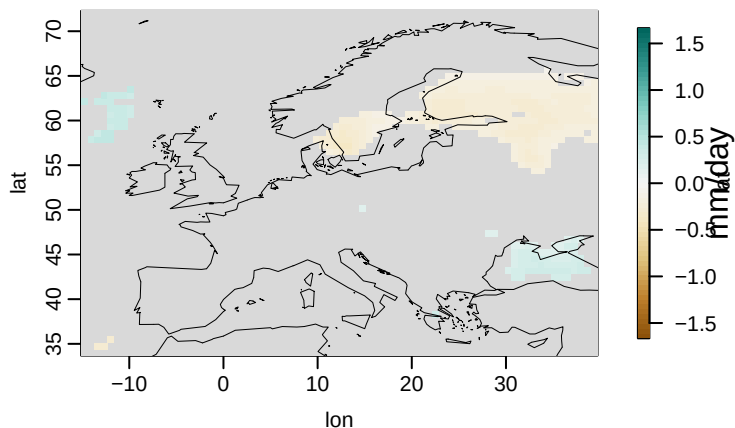
HadGEM3-GC31-LL u03
