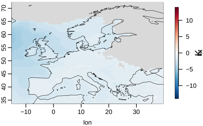
HadGEM3-GC31-MM g01
