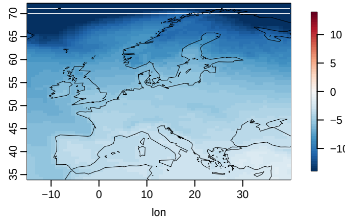
HadGEM3-GC31-MM u03
