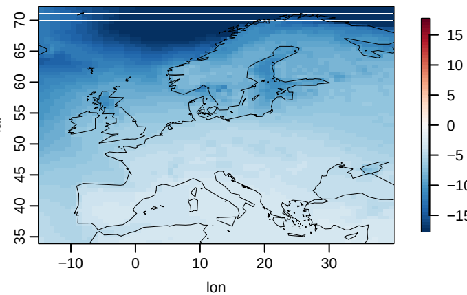
HadGEM3-GC31-MM u03
