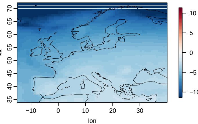
HadGEM3-GC31-MM u03
