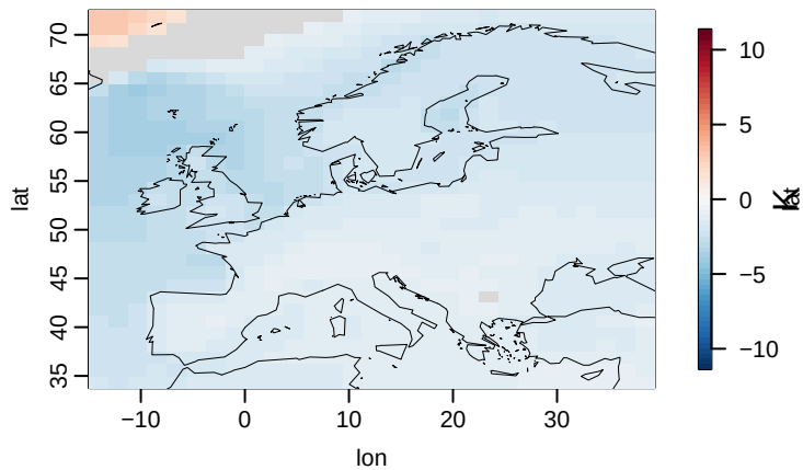
IPSL-CM6A-LR u03
