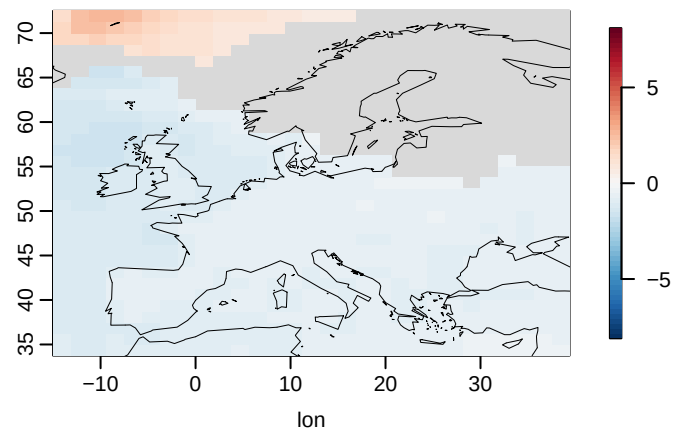
HadGEM3-GC31-MM u03
