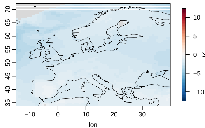
HadGEM3-GC31-MM g01
