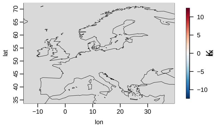
HadGEM3-GC31-LL u03
