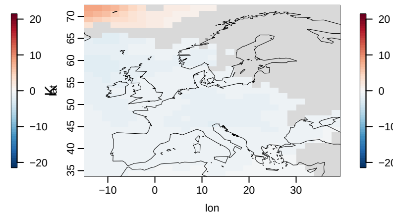
HadGEM3-GC31-MM u03
