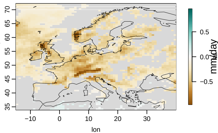
HadGEM3-GC31-MM g01
