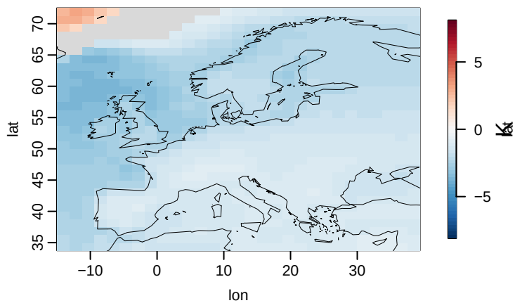
IPSL-CM6A-LR u03
