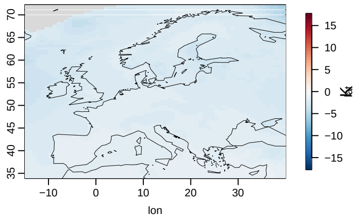
HadGEM3-GC31-MM g01
