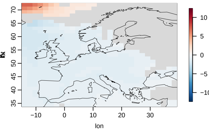
HadGEM3-GC31-MM u03
