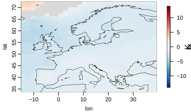
IPSL-CM6A-LR u03
