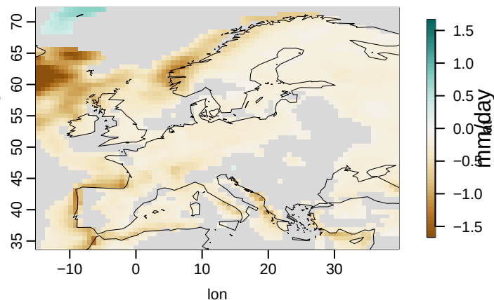
HadGEM3-GC31-MM g01
