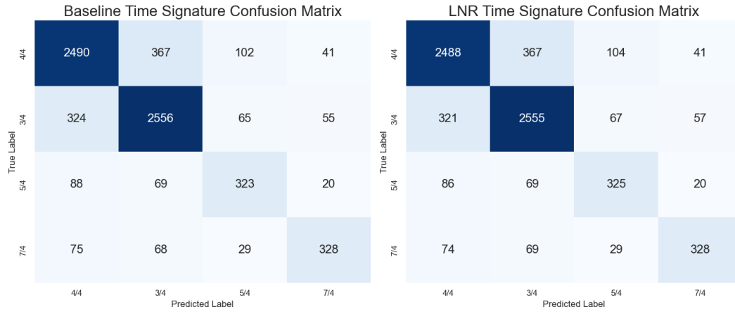
Figure 2: LNR confusion matrices on Meter2800 test data with t_{flip} = 7 , epochs = 140.
