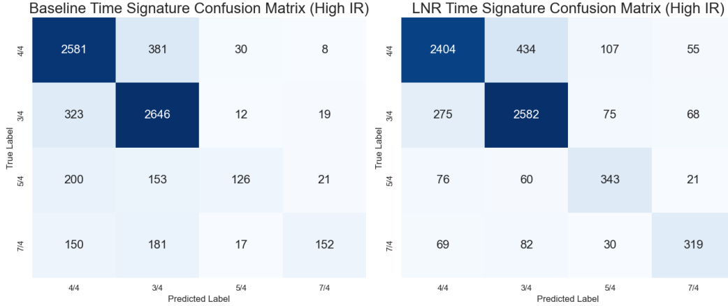
Figure 1: LNR confusion matrices on Meter2800 test data with t_{flip} = 7 , epochs = 100 (high IR).
