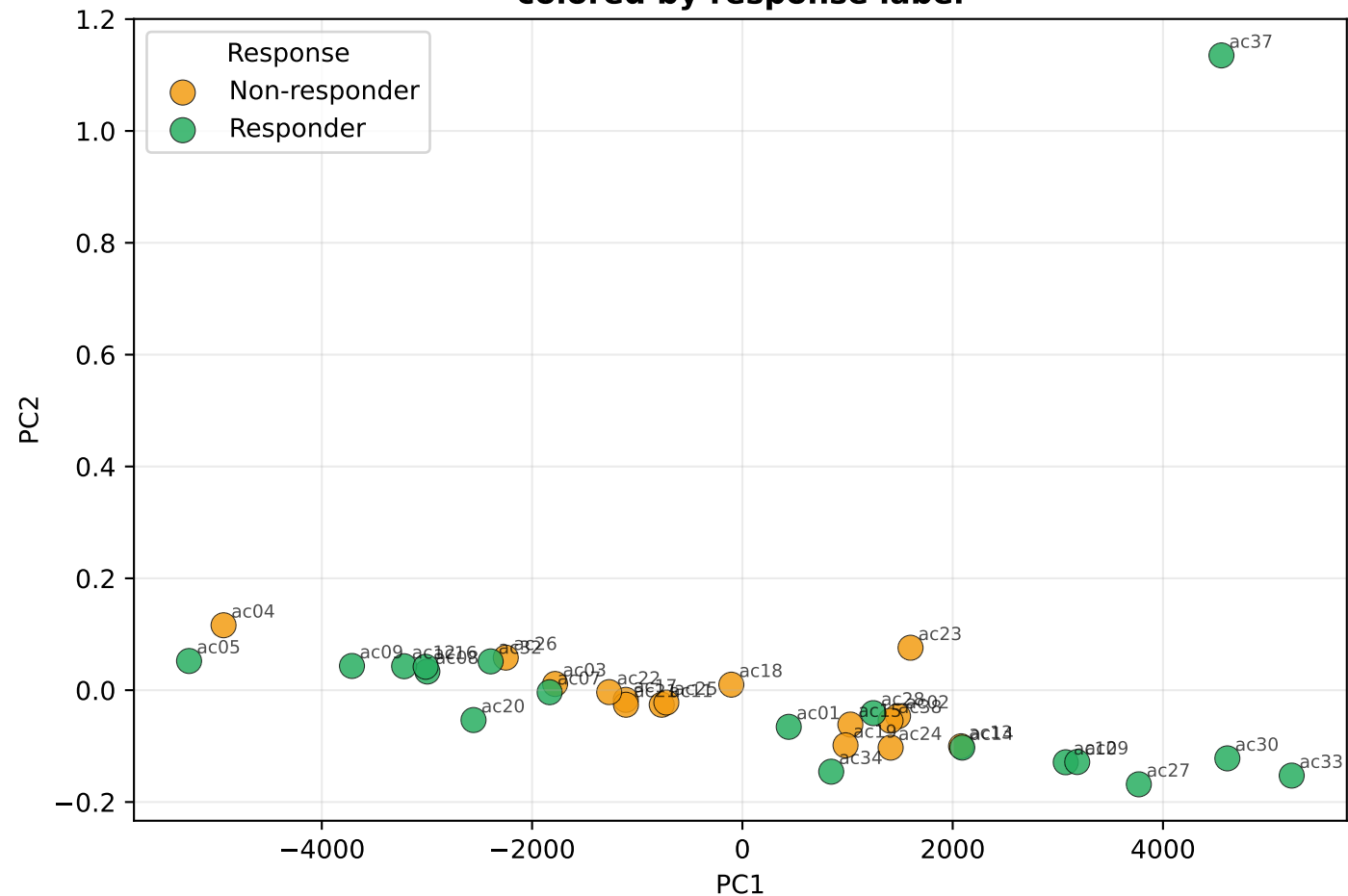
Figure S10: Unsupervised patient embedding (PCA) colored by response label
