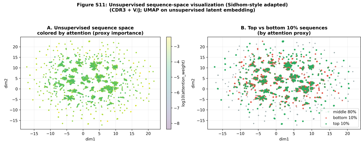
Figure 18: Unsupervised Sequence-Space Visualization. A two-dimensional visualization of an unsupervised latent embedding of TRB sequences derived from CDR3 k-mer features and V/J gene usage. Points are colored by attention-based importance (proxy for “predictive” sequences) and top vs. bottom deciles highlight enrichment of high-importance sequences within specific regions of sequence space, analogous to unsupervised visualization strategies used in DeepTCR studies.
