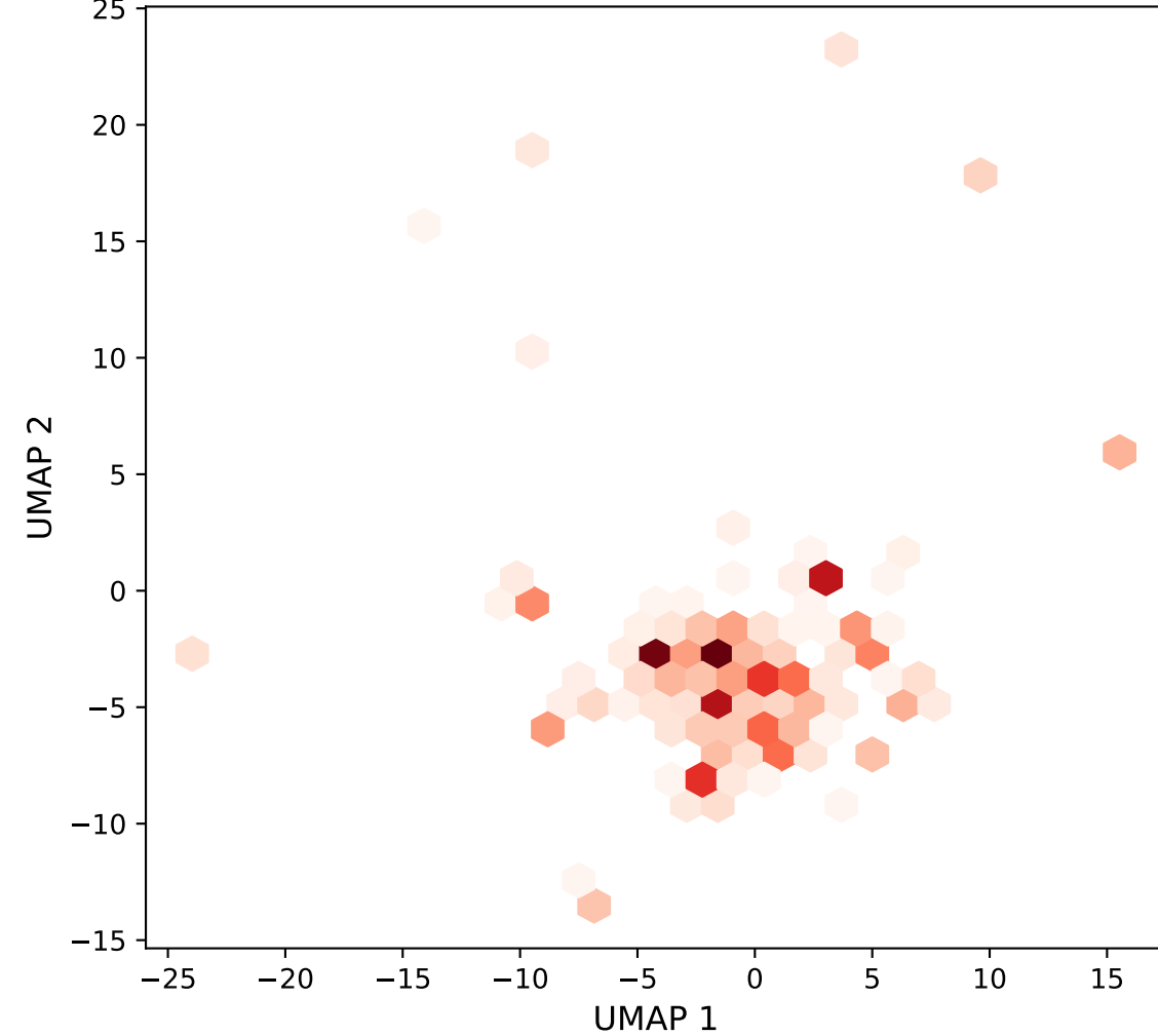
C. Non-responder TCR Distribution (Density)
