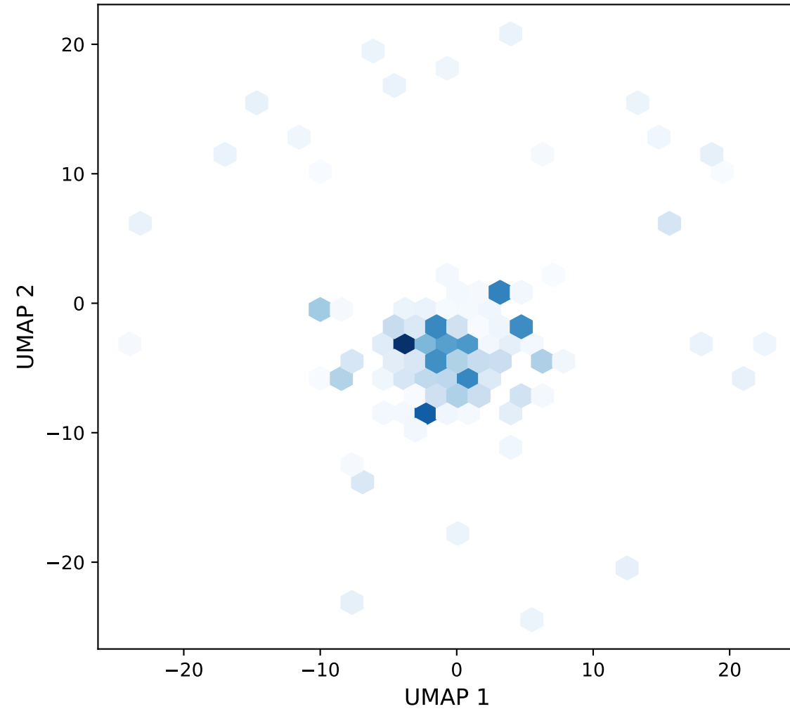
B. Responder TCR Distribution (Density)
