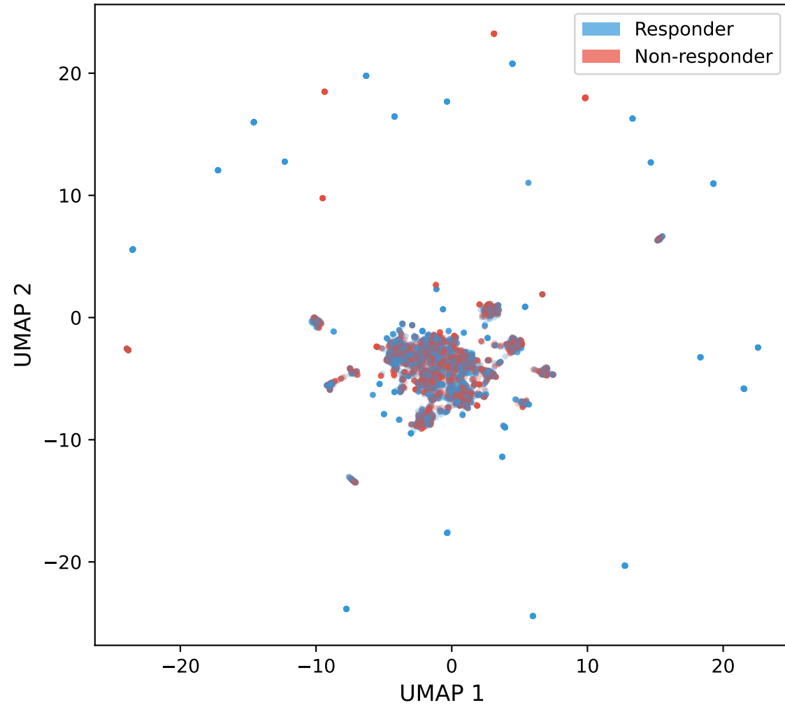
A. TCR Repertoire Distribution (All Sequences)
