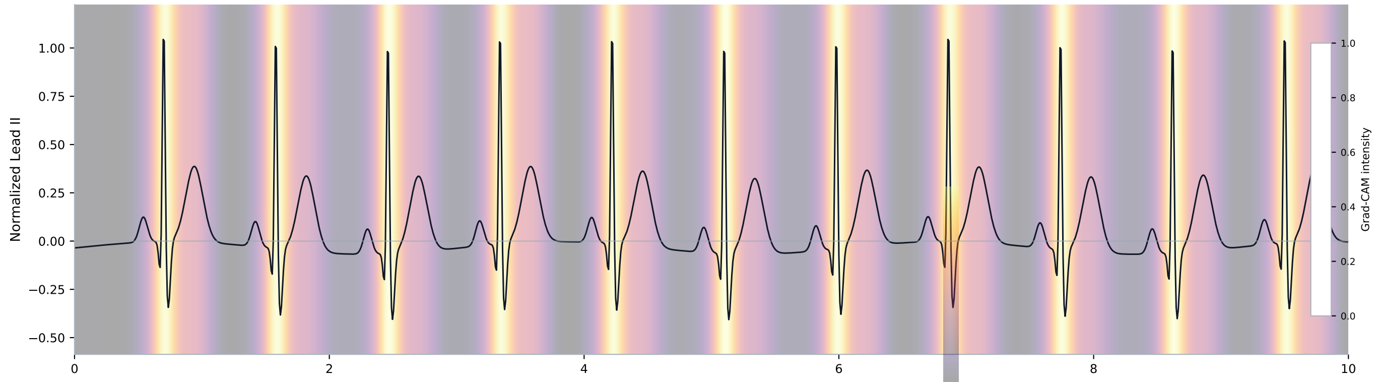
Lead-time Grad-CAM intensity map
