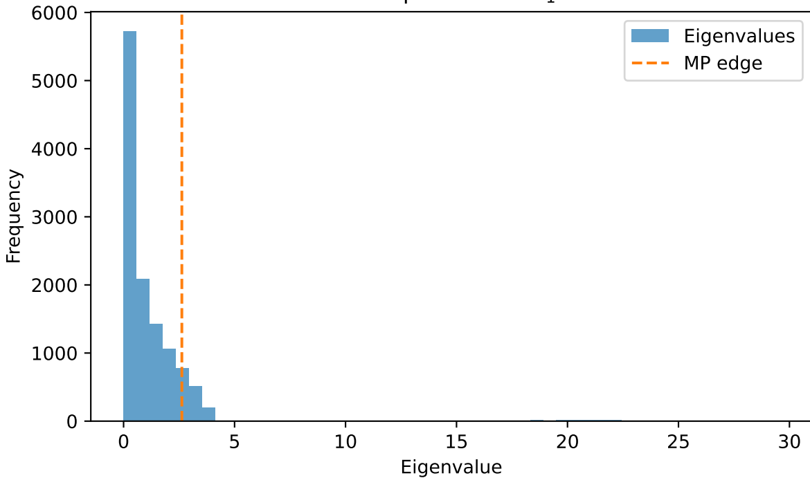
S1: Spectrum of \Sigma_1
