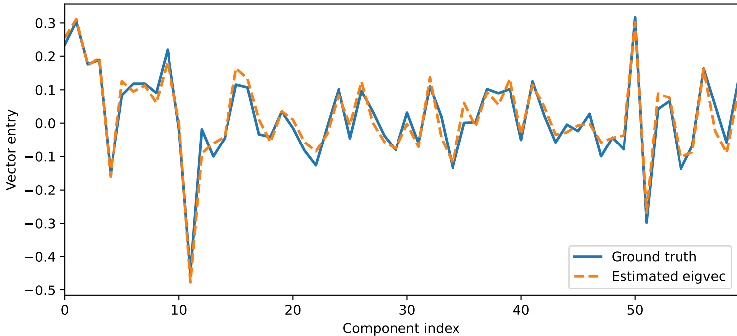
S2: Leading eigenvector alignment (cosine=0.971)
