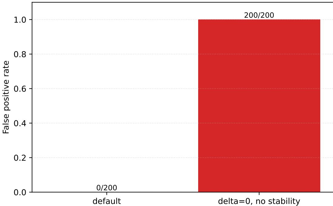
S4: Guardrail comparison on isotropic data
