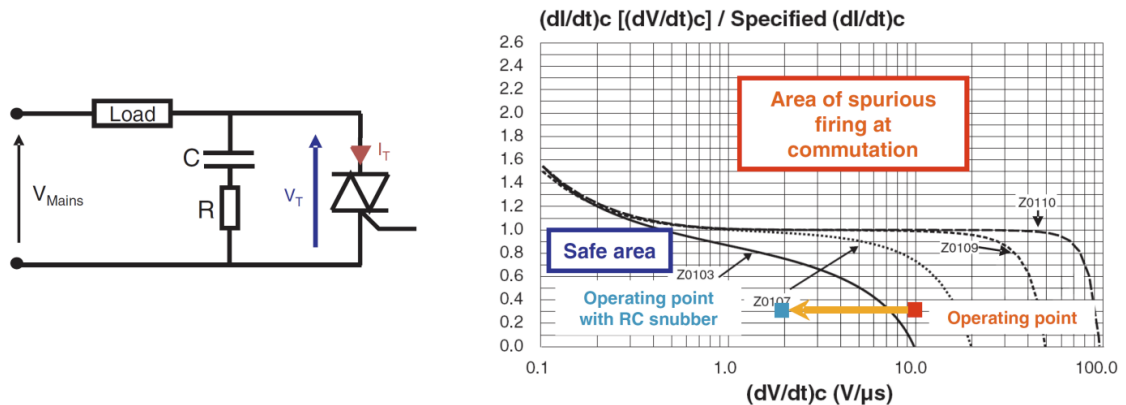
Figura 22: Red Snubber.
