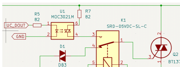
Figura 7: Driver TRIAC.
