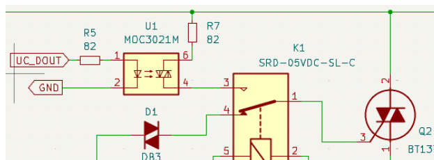
Figura 7: Driver TRIAC.
