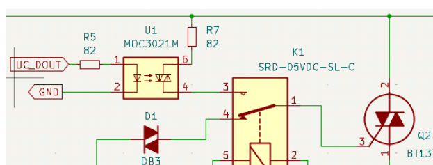
Figura 9: Driver TRIAC.
