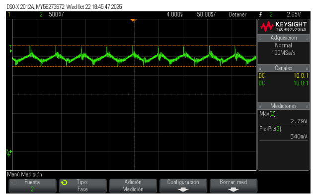
(b) Capacitor.
