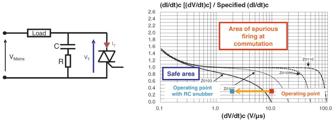
Figura 23: Red Snubber.
