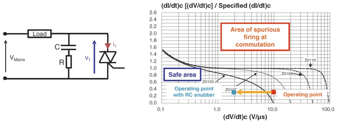
Figura 9: Red Snubber.
