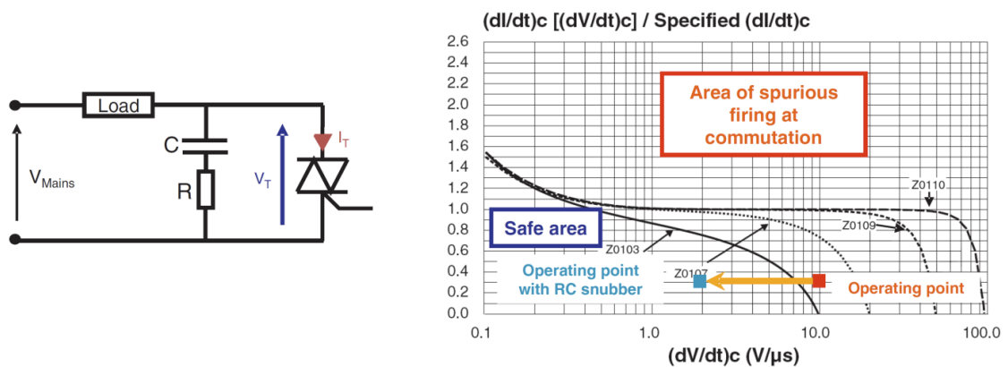
Figura 22: Red Snubber.
