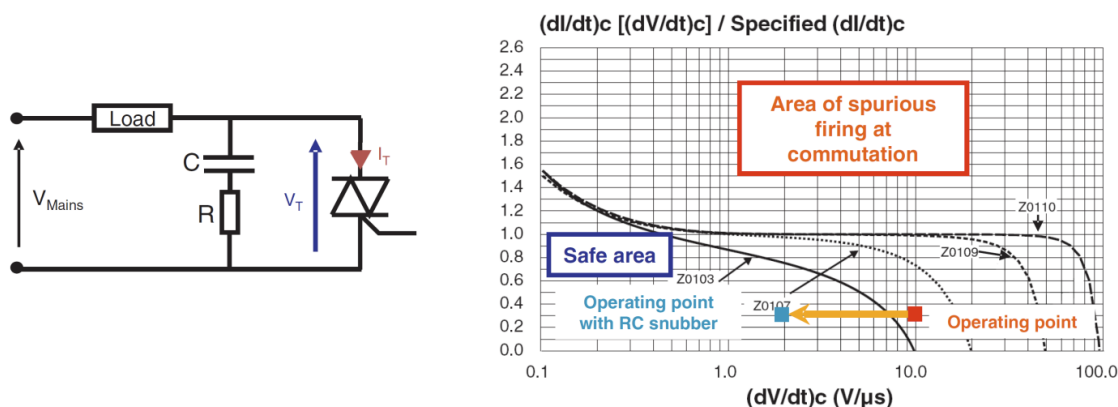
Figura 22: Red Snubber.
