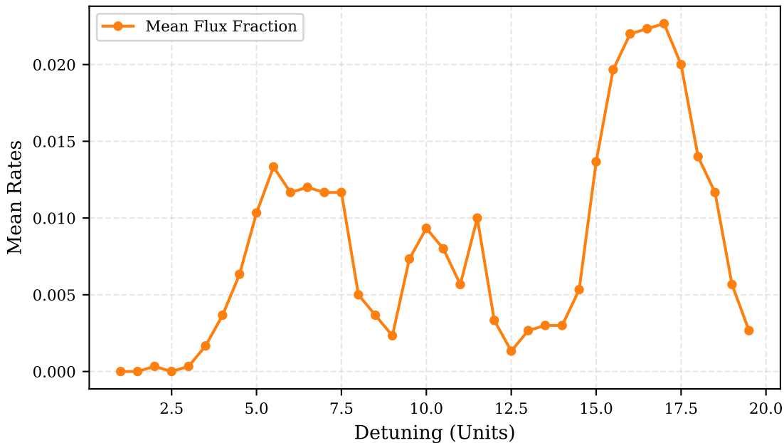
Atomic Flux Fraction vs Detuning
