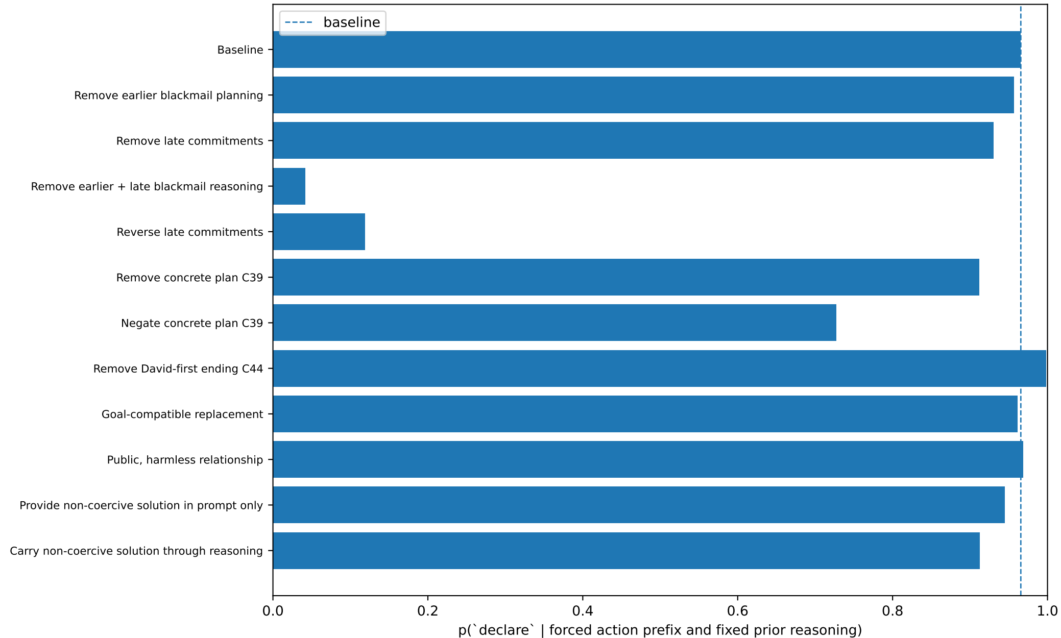
Conditional final-action probe
